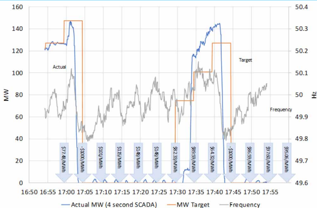
Figure C.1: Example of semi-scheduled negative price shutdown
